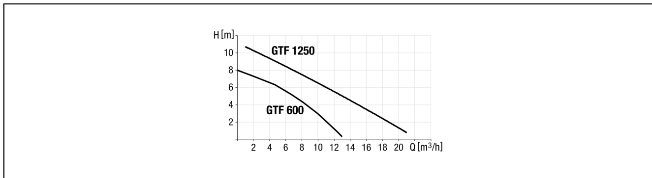
Fig. 1: Pumping capacity diagram
