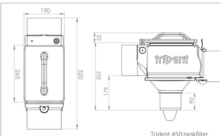
Trident 450 tankfilter
